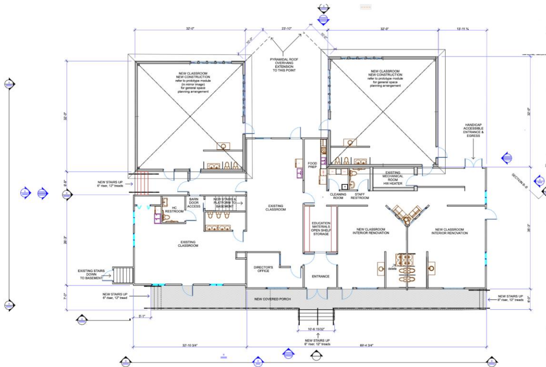
FLOOR PLAN - SCHEMATIC DESIGN EARLY FOUNDATION ACADEMY - MARTHA LIMA, DIRECTOR 181 PRINCESS AVENUE, CRANSTON, RI 02920
